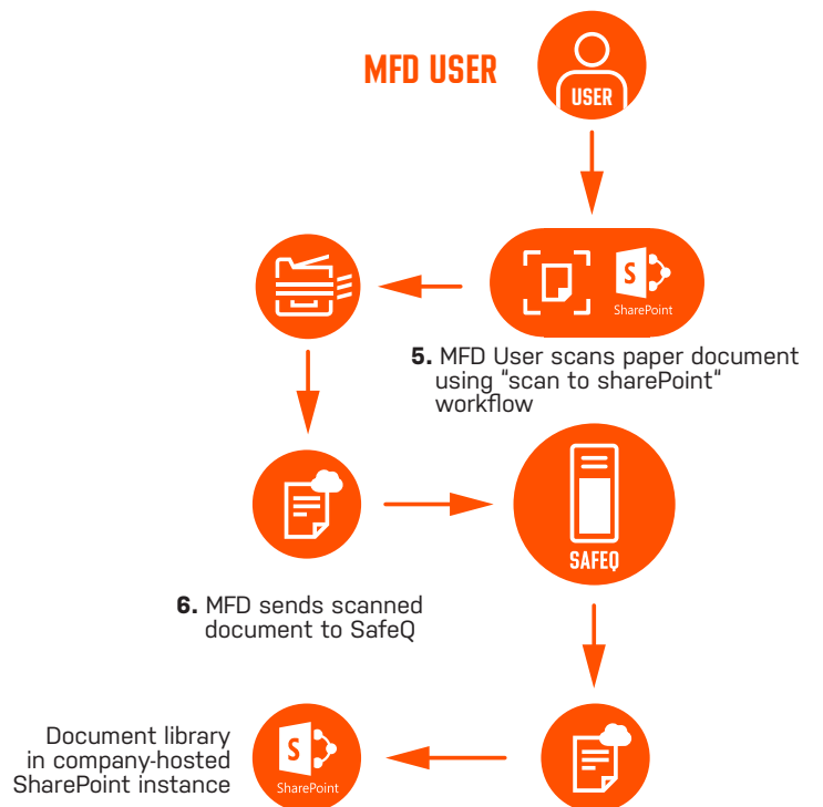
Figure 6. Simple workflow sends scans to pre-defined locations such as SharePoint or Dropbox.
