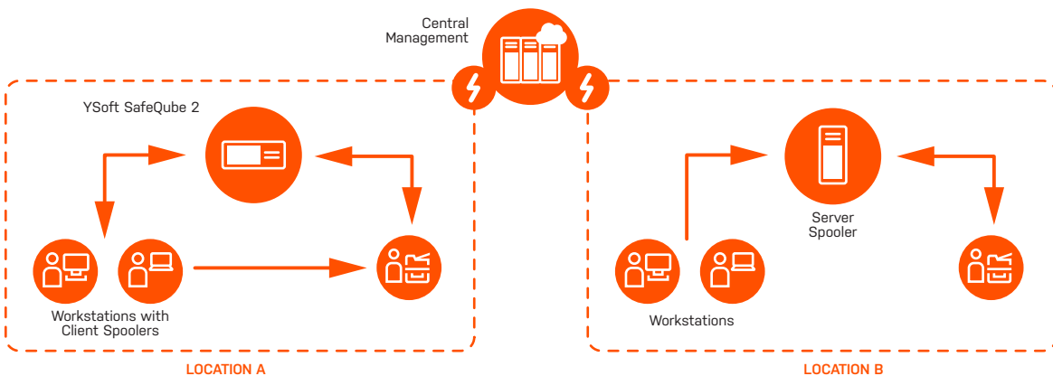
Figure 3. Client Based Print Roaming with optional YSoft SafeQube 2 appliance
