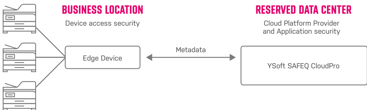
Figure 1 YSoft SAFEQ CloudPro Metadata Flow
